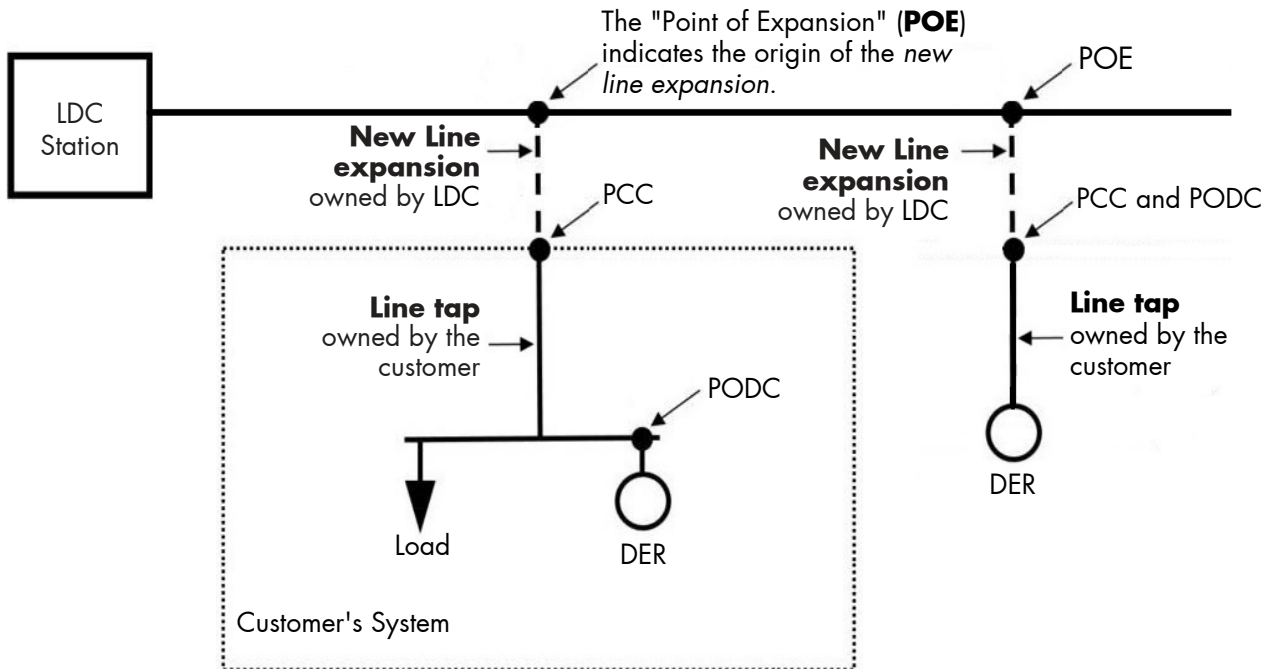
Figure A2: Where there is a New Atikokan Hydro Owned Line Expansion
