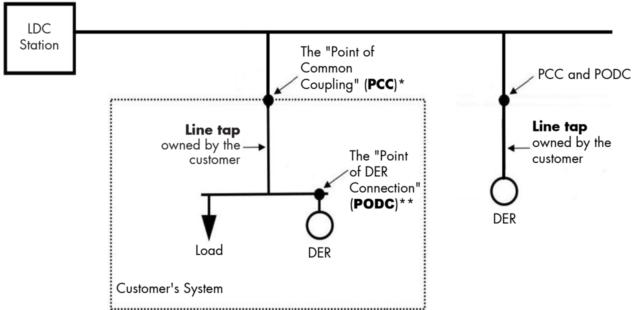
Figure A1: Where there is No New Atikokan Hydro Owned Line Expansion
